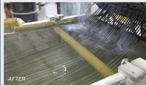
Extrusion baths before and after installation of Armstrong Nanobubble Generator (3/4"x1.5").
