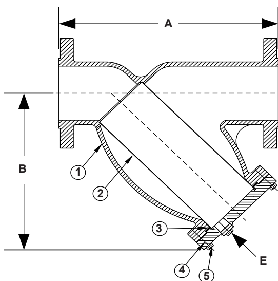
Cast 316 Stainless Steel Y-Strainer
