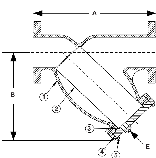
Cast Carbon Steel Y-Strainer
