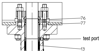
Graphite EN ISO 15848-1 with O-Rings and test port
