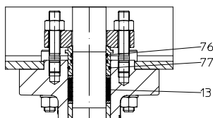
Graphite EN ISO 15848-1 with O-Rings
