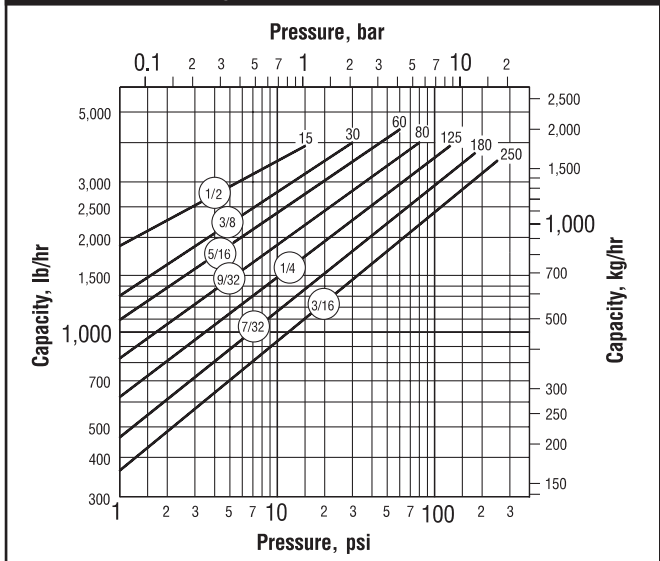
Model 883 Capacity
