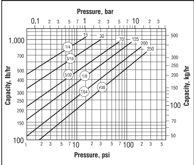
Model 881 Capacity
