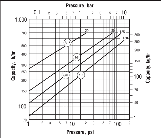
Model 880 Capacity
