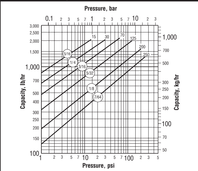
Model 882 Capacity
