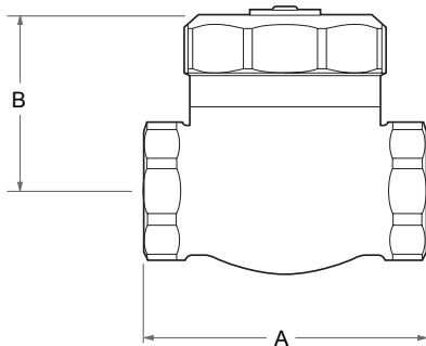
Bronze horizontal lift check valve Female ends, PN32
