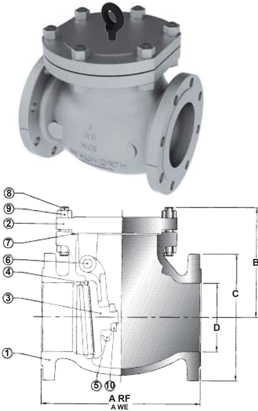
Figure No. Type of Ends 5344RF Flanged Raised Face
