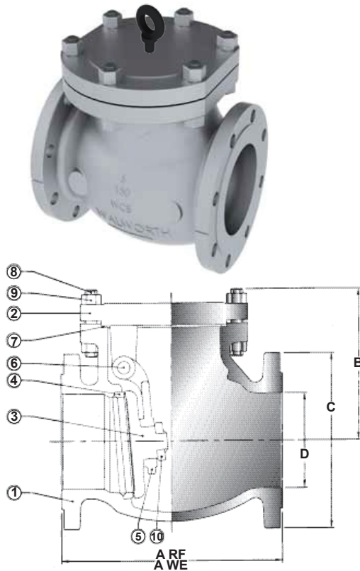
Figure No. Type of Ends 5341RF Flanged Raised Face
